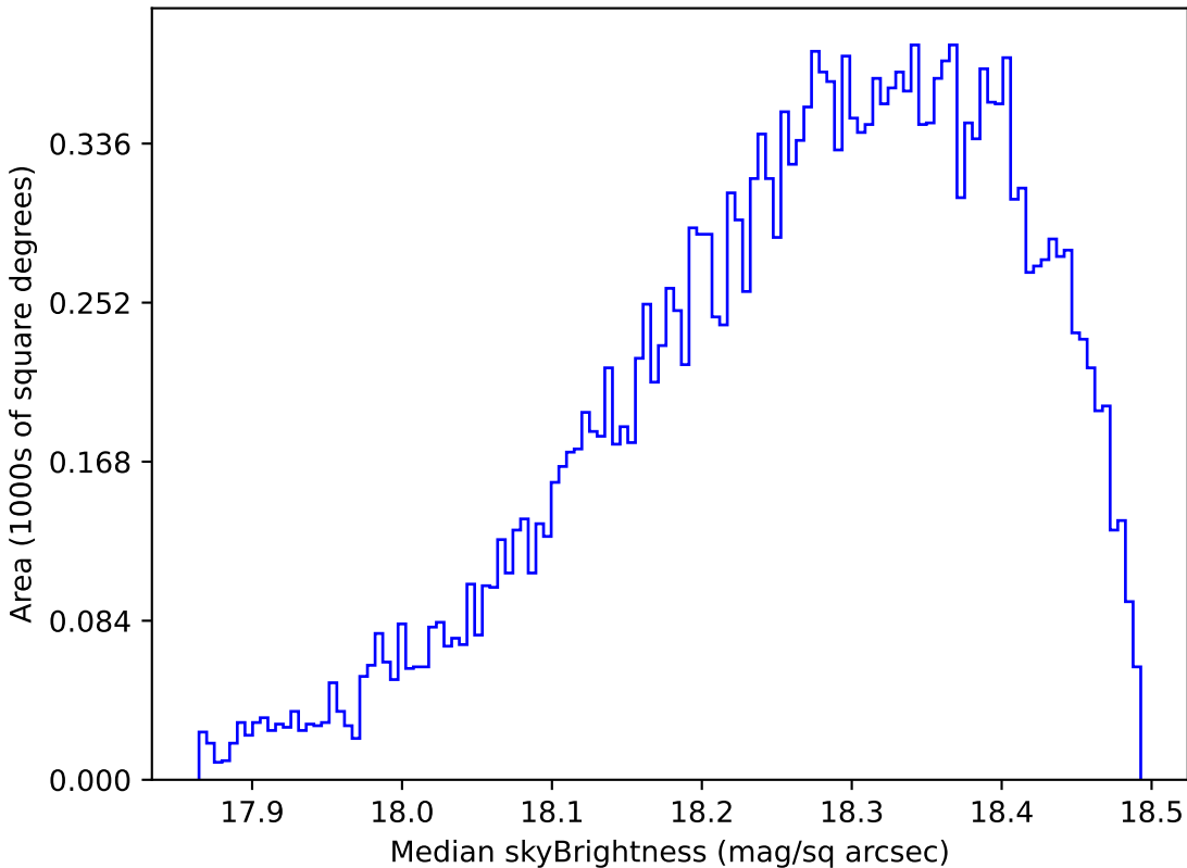
smc_lmc_v3.3_10yrs Yr 1 y band: Median skyBrightness
