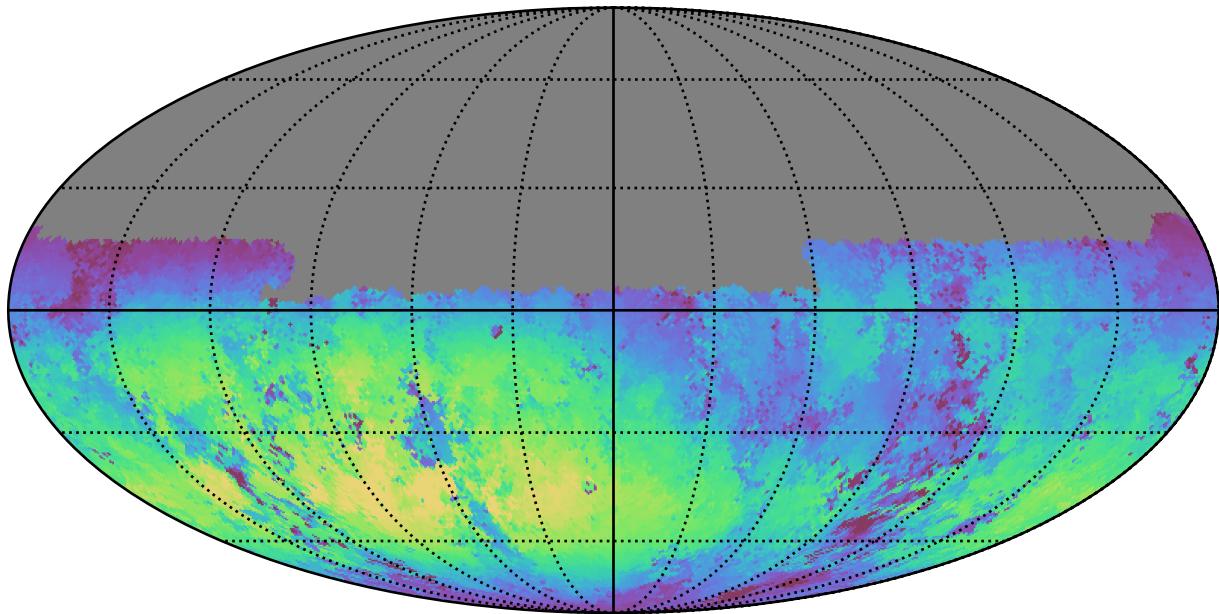
smc_lmc_v3.3_10yrs Yr 1 u band: Median skyBrightness
