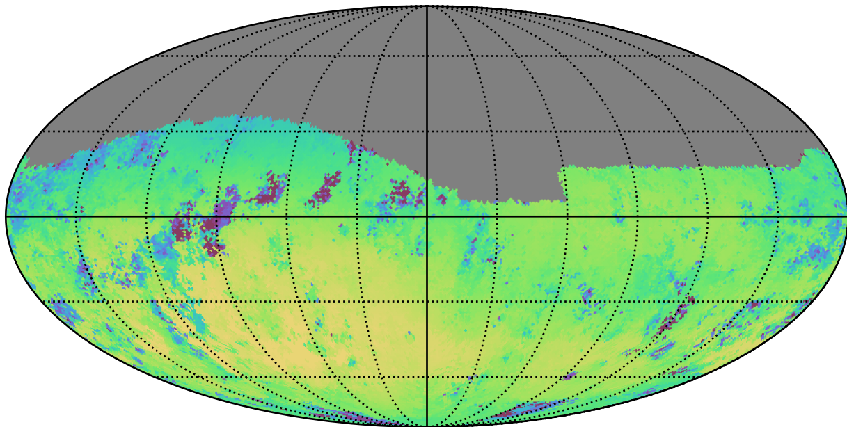
smc_lmc_v3.3_10yrs Yr 1 r band: Median skyBrightness
