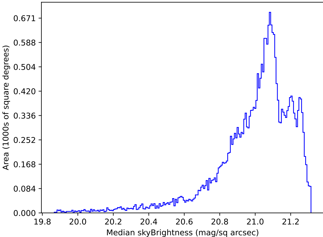
smc_lmc_v3.3_10yrs Yr 1 r band: Median skyBrightness
