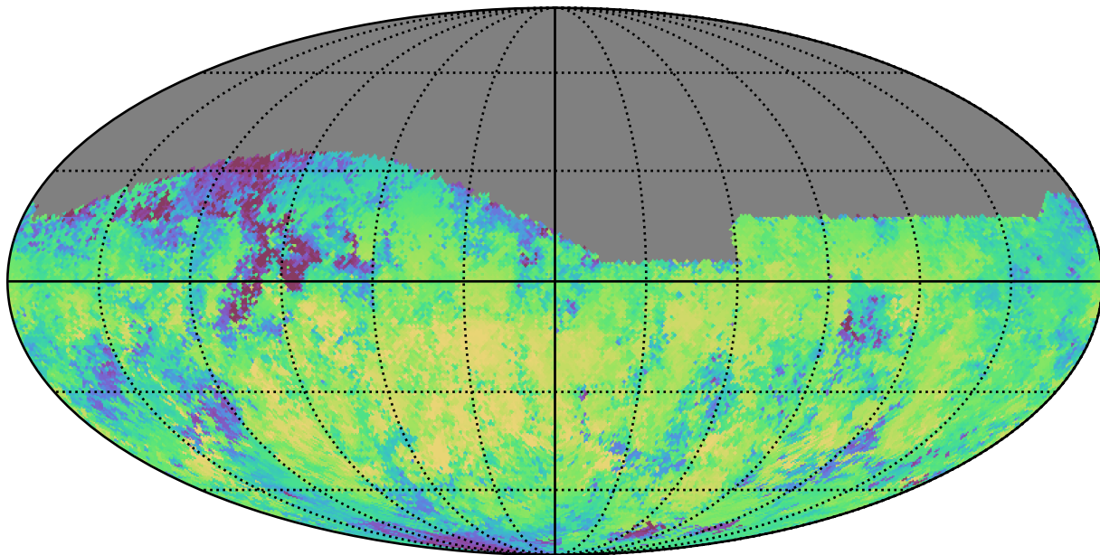
smc_lmc_v3.3_10yrs Yr 1 i band: Median skyBrightness
