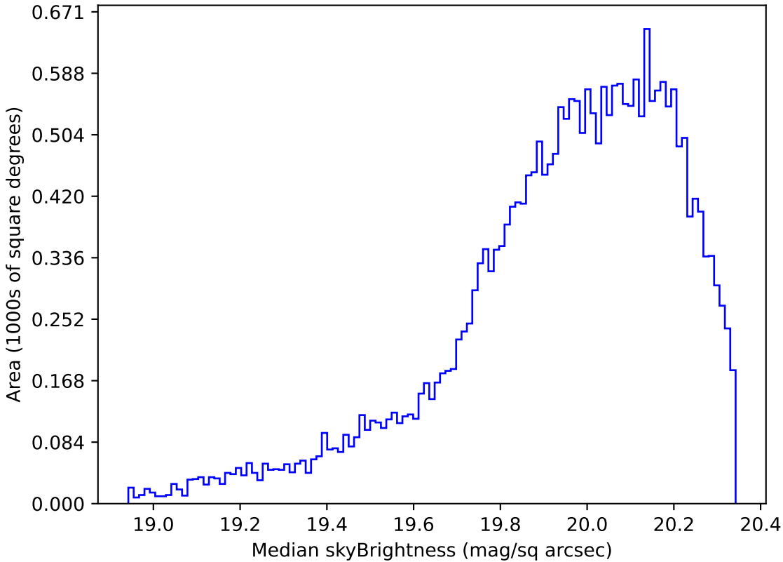
smc_lmc_v3.3_10yrs Yr 1 i band: Median skyBrightness
