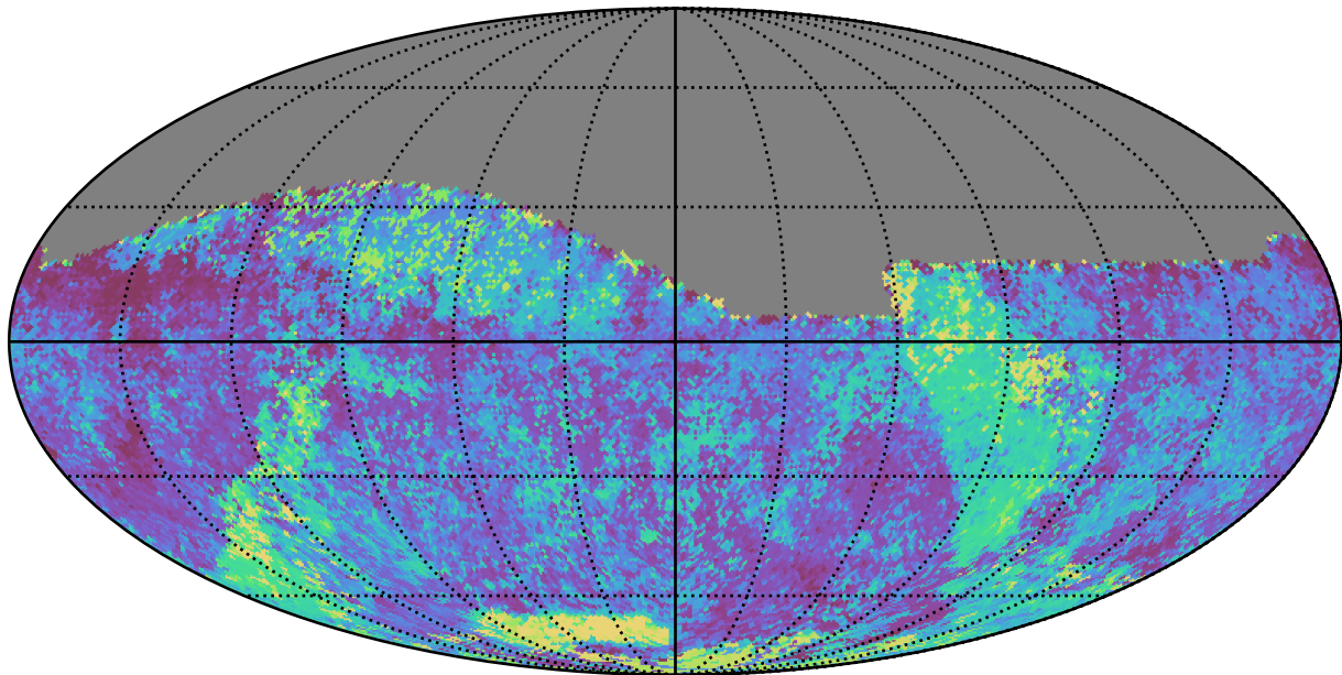
smc_lmc_v3.3_10yrs Yr 1 all bands: Median skyBrightness
