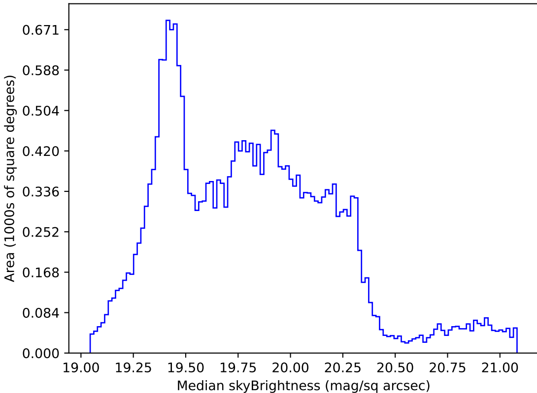
smc_lmc_v3.3_10yrs Yr 1 all bands: Median skyBrightness
