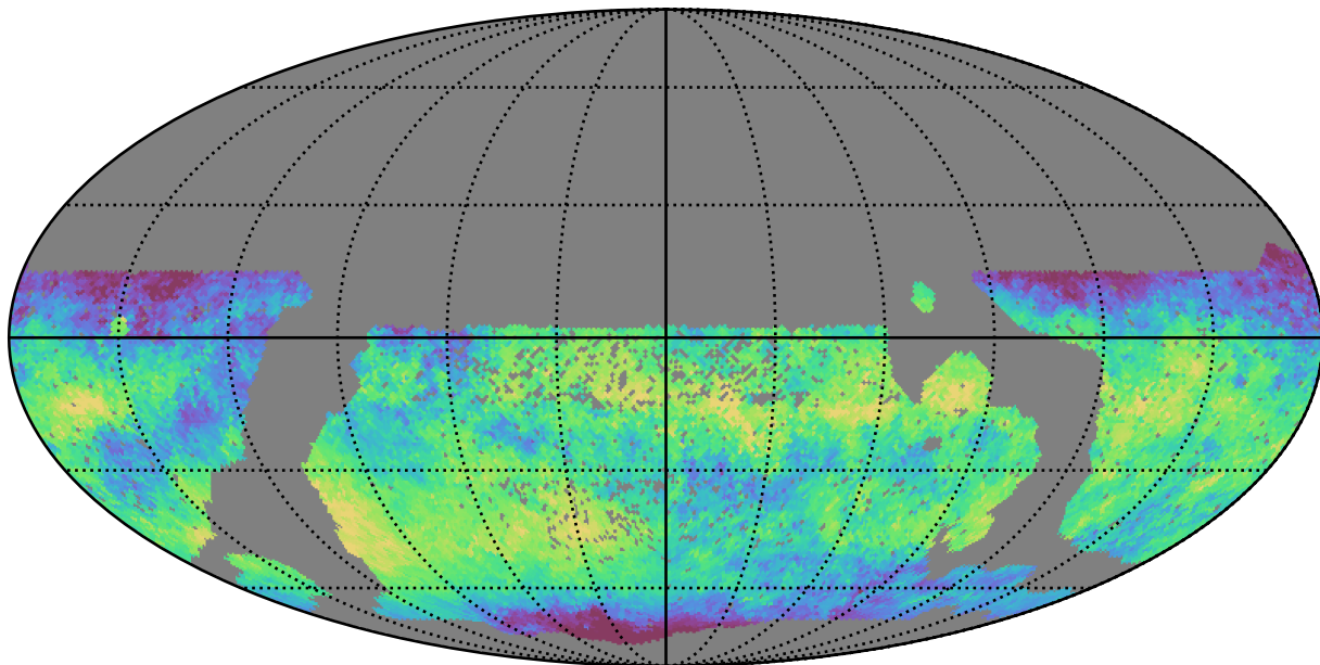
smc_lmc_v3.3_10yrs WFD z band: Median skyBrightness
