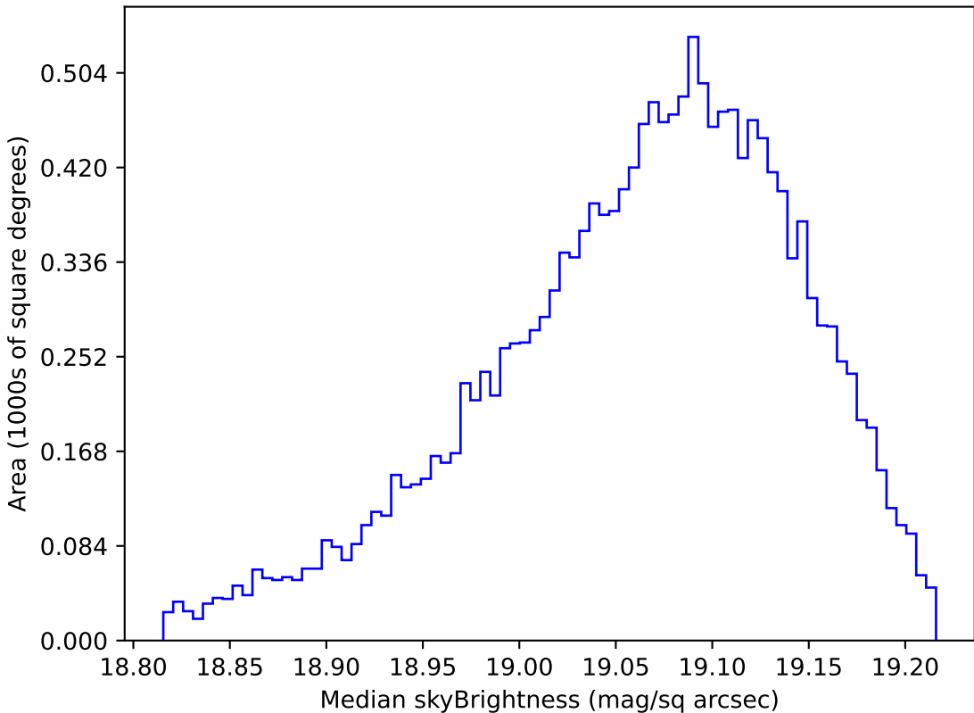
smc_lmc_v3.3_10yrs WFD z band: Median skyBrightness
