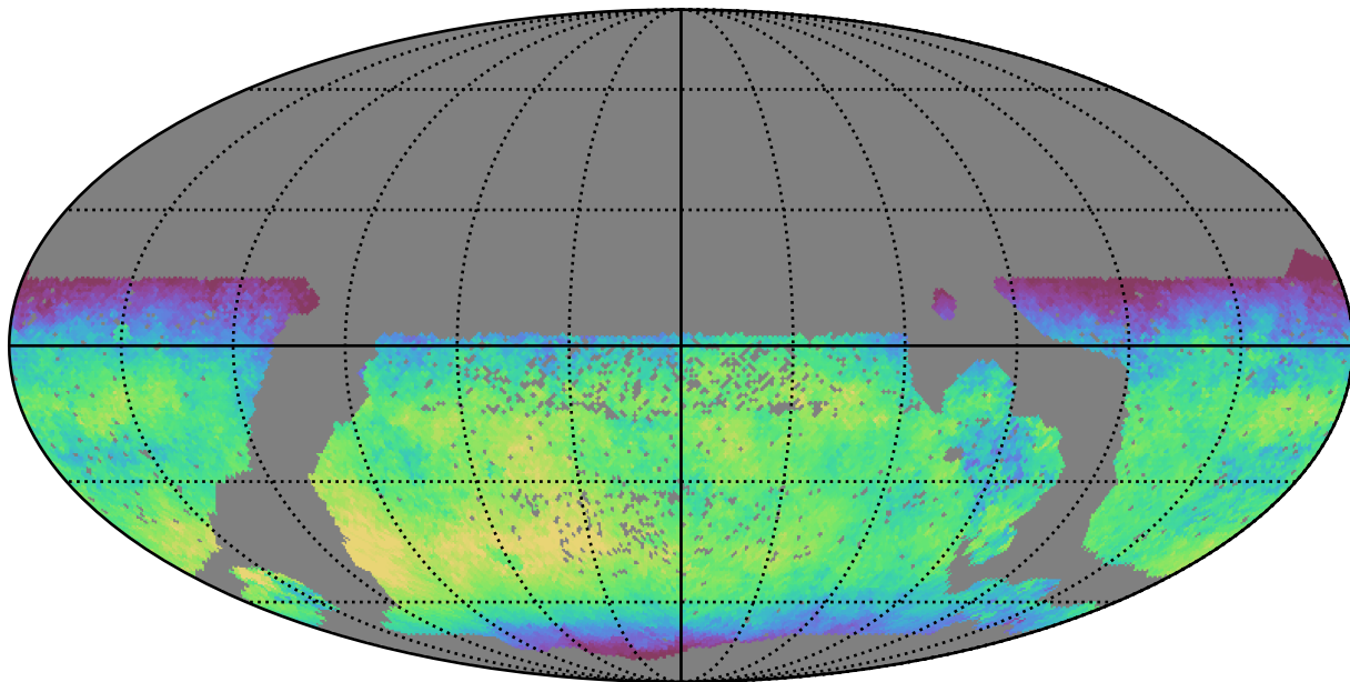
smc_lmc_v3.3_10yrs WFD y band: Median skyBrightness
