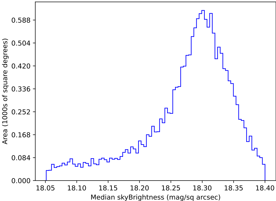
smc_lmc_v3.3_10yrs WFD y band: Median skyBrightness
