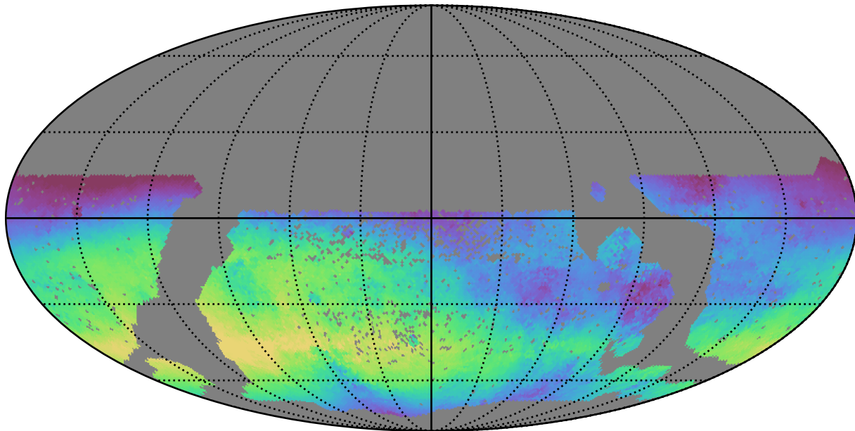
smc_lmc_v3.3_10yrs WFD u band: Median skyBrightness
