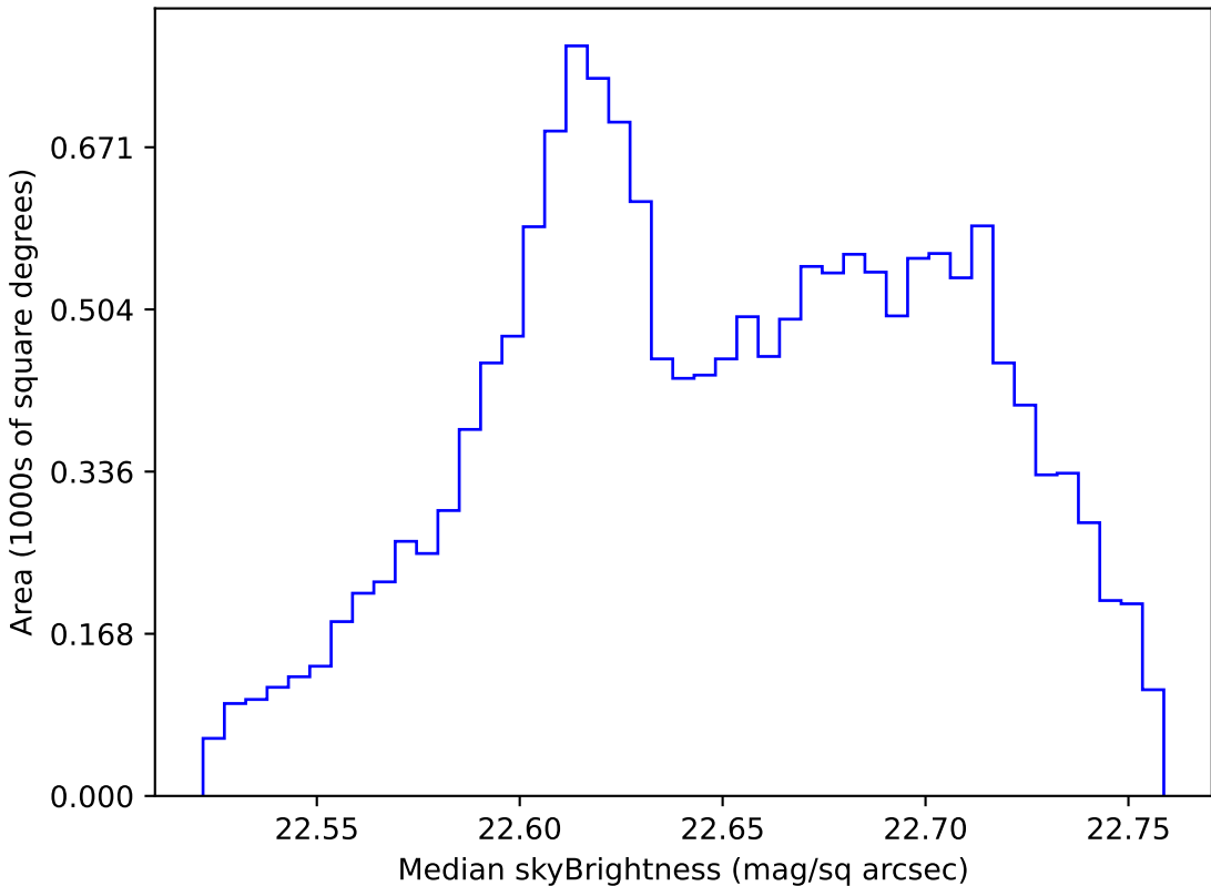
smc_lmc_v3.3_10yrs WFD u band: Median skyBrightness
