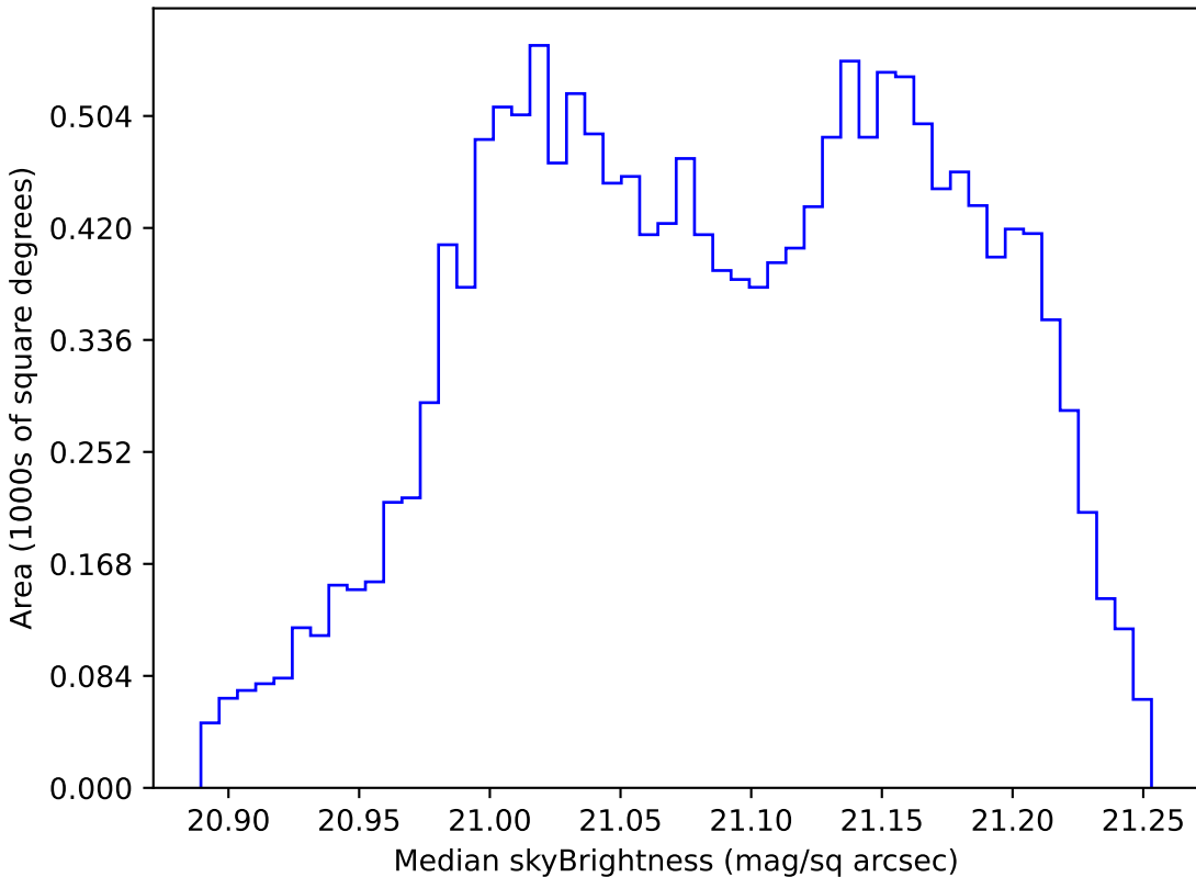
smc_lmc_v3.3_10yrs WFD r band: Median skyBrightness
