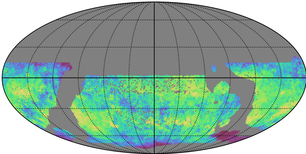
smc_lmc_v3.3_10yrs WFD i band: Median skyBrightness
