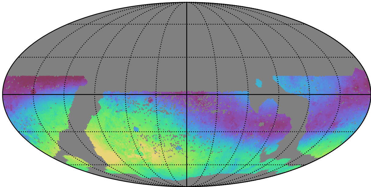
smc_lmc_v3.3_10yrs WFD g band: Median skyBrightness
