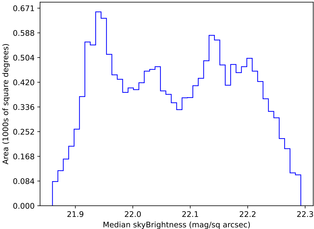
smc_lmc_v3.3_10yrs WFD g band: Median skyBrightness
