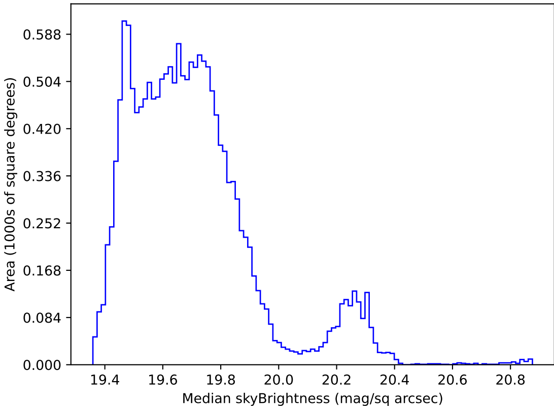
smc_lmc_v3.3_10yrs WFD all bands: Median skyBrightness
