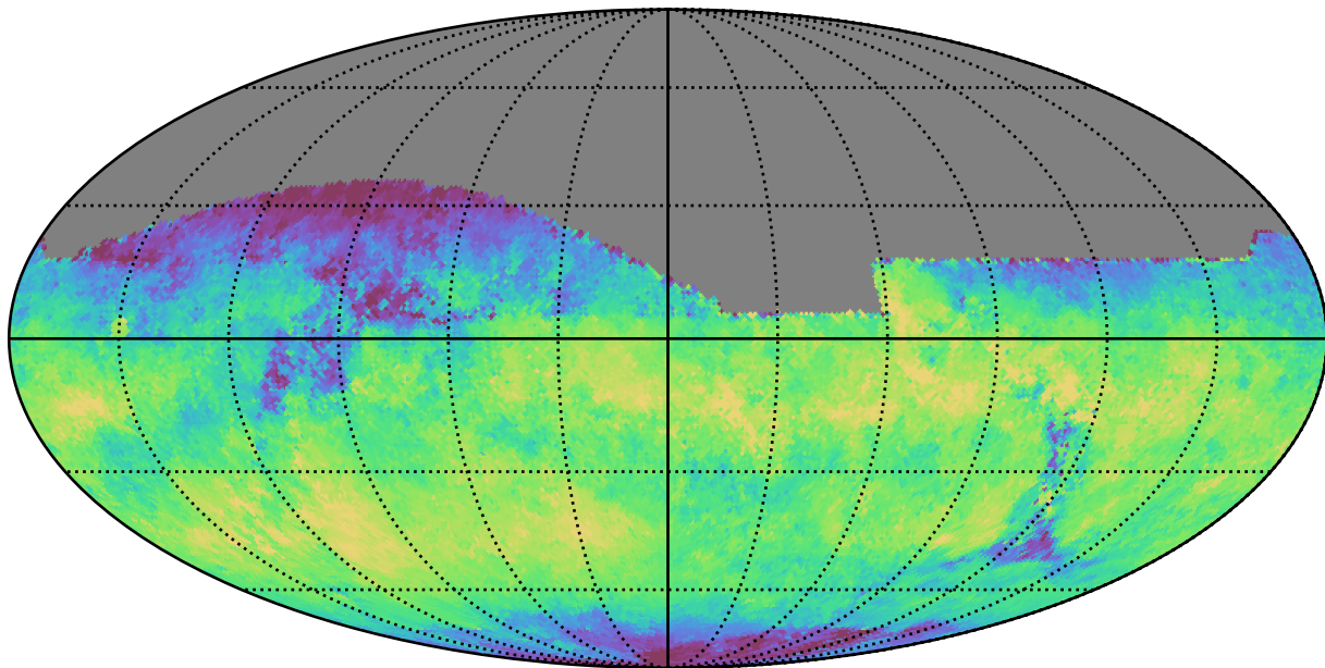
smc_lmc_v3.3_10yrs All sky z band: Median skyBrightness
