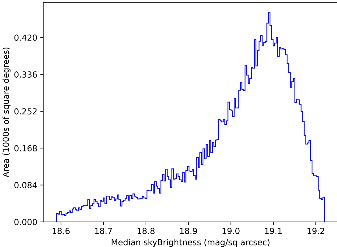
smc_lmc_v3.3_10yrs All sky z band: Median skyBrightness
