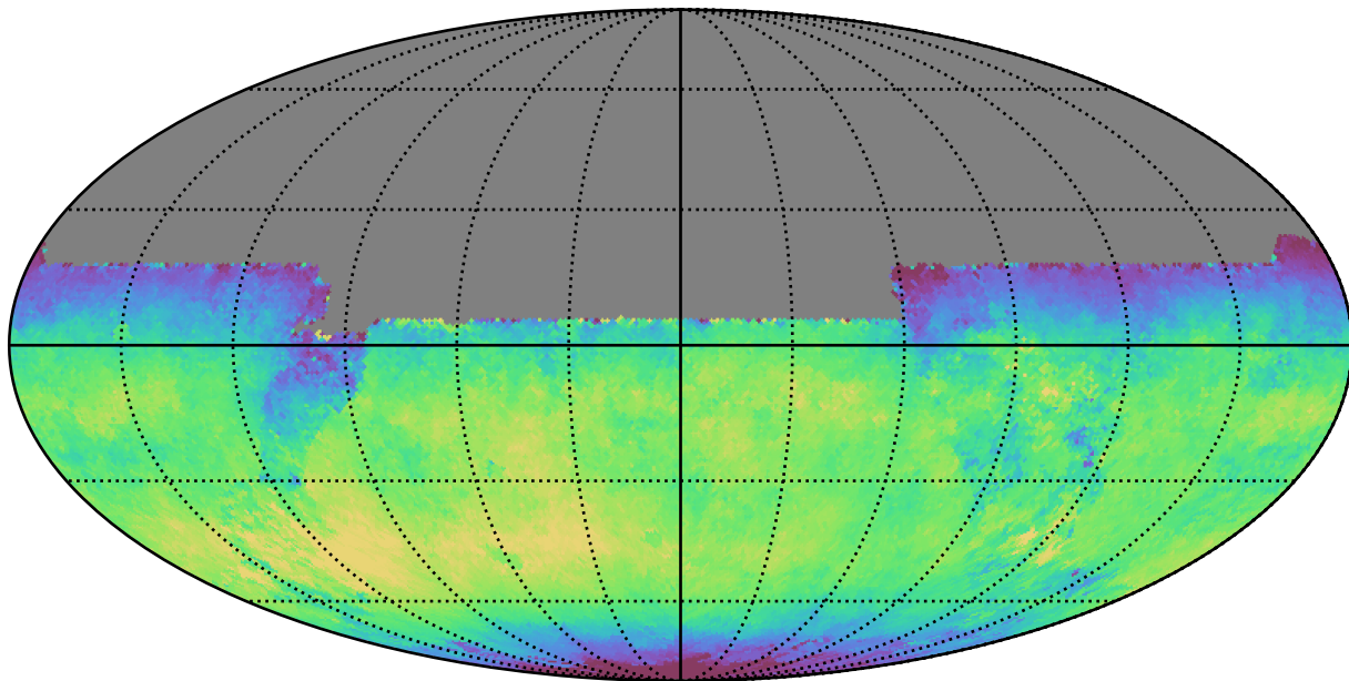
smc_lmc_v3.3_10yrs All sky y band: Median skyBrightness
