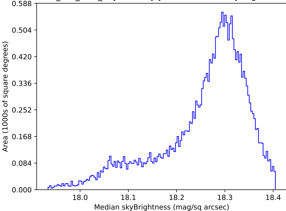
smc_lmc_v3.3_10yrs All sky y band: Median skyBrightness
