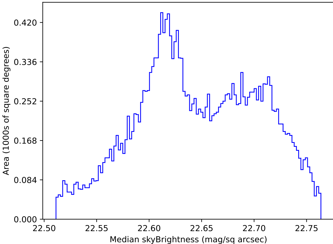
smc_lmc_v3.3_10yrs All sky u band: Median skyBrightness
