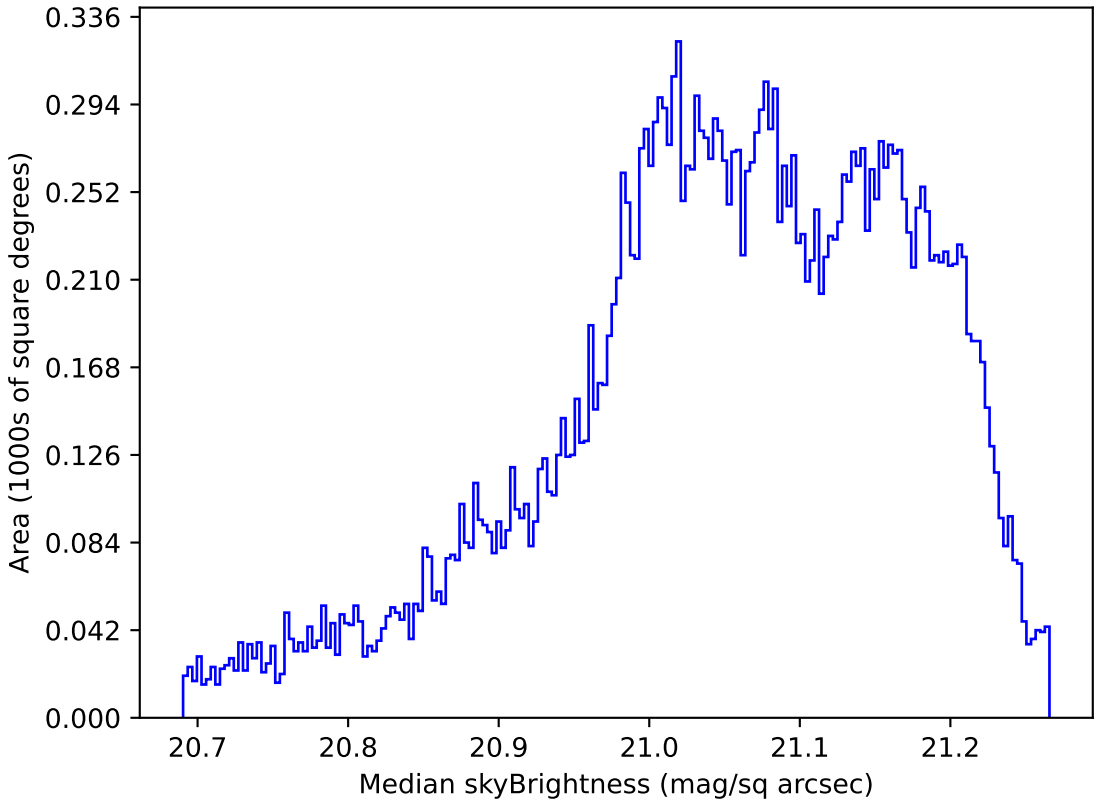
smc_lmc_v3.3_10yrs All sky r band: Median skyBrightness
