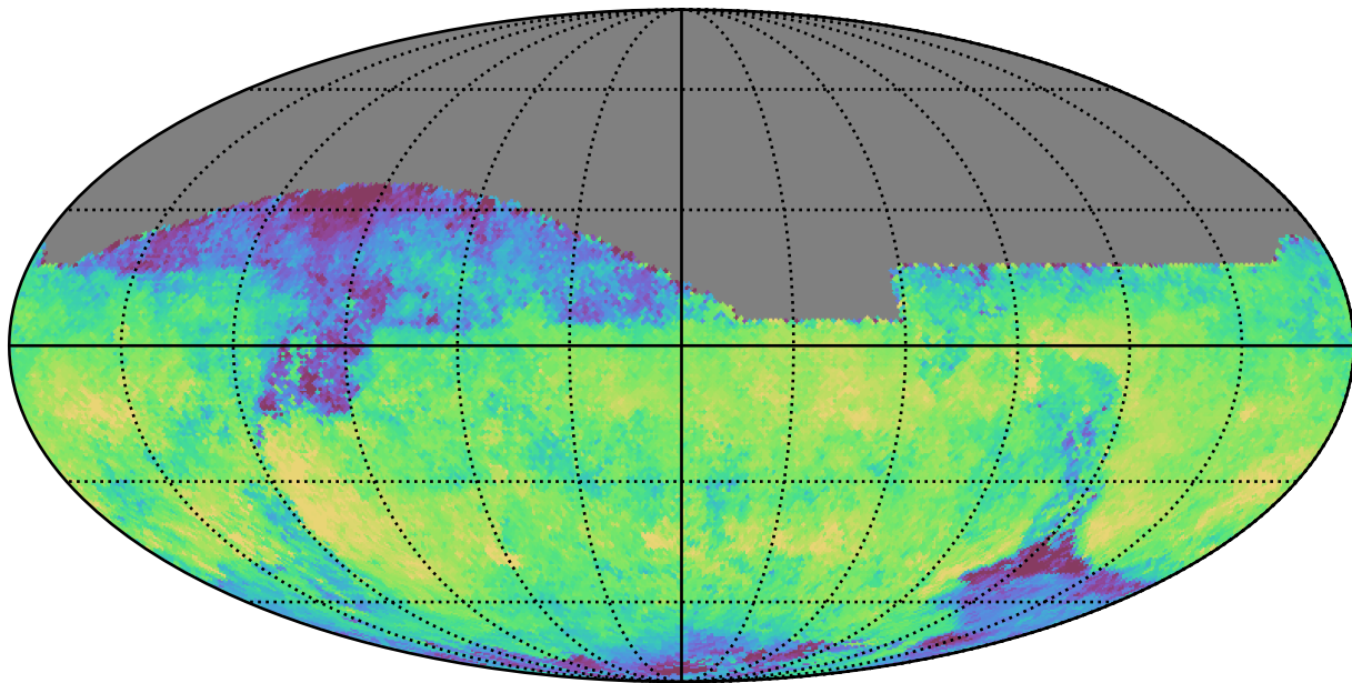
smc_lmc_v3.3_10yrs All sky i band: Median skyBrightness
