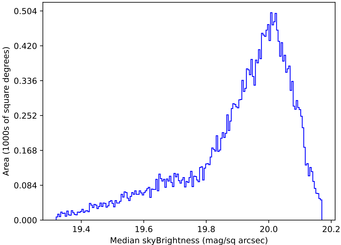
smc_lmc_v3.3_10yrs All sky i band: Median skyBrightness
