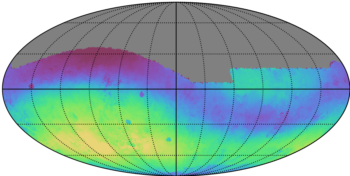
smc_lmc_v3.3_10yrs All sky g band: Median skyBrightness
