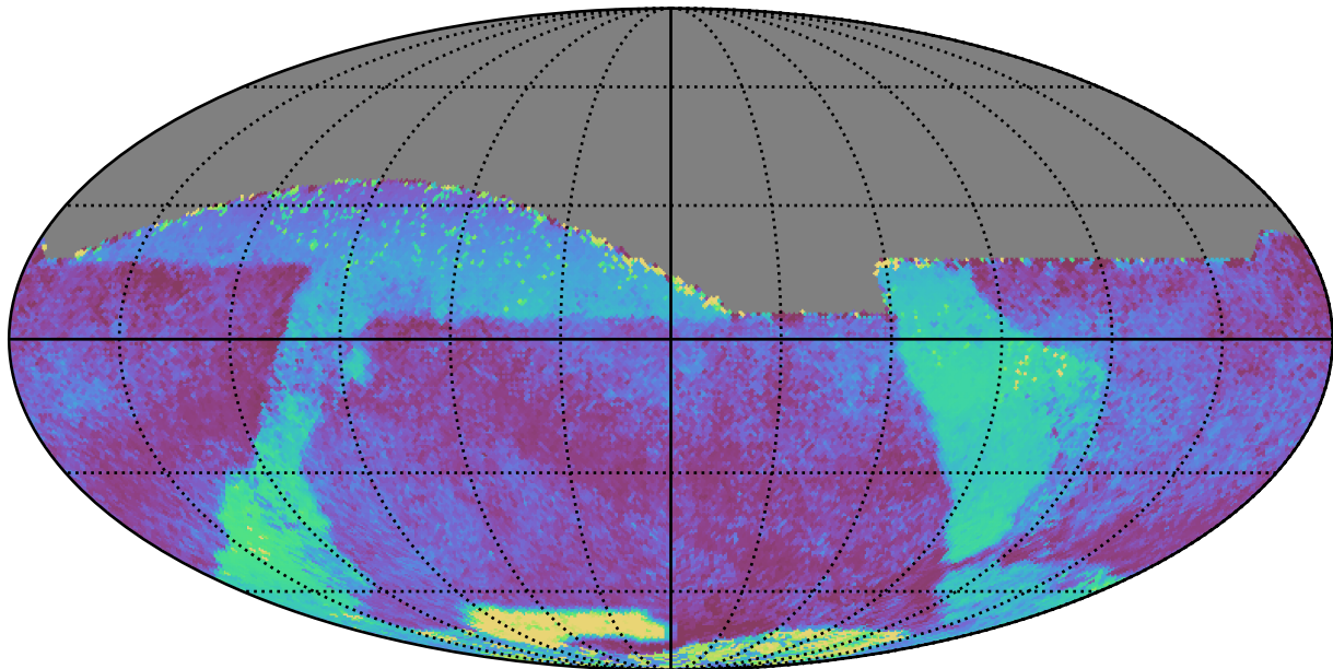
smc_lmc_v3.3_10yrs All sky all bands: Median skyBrightness
