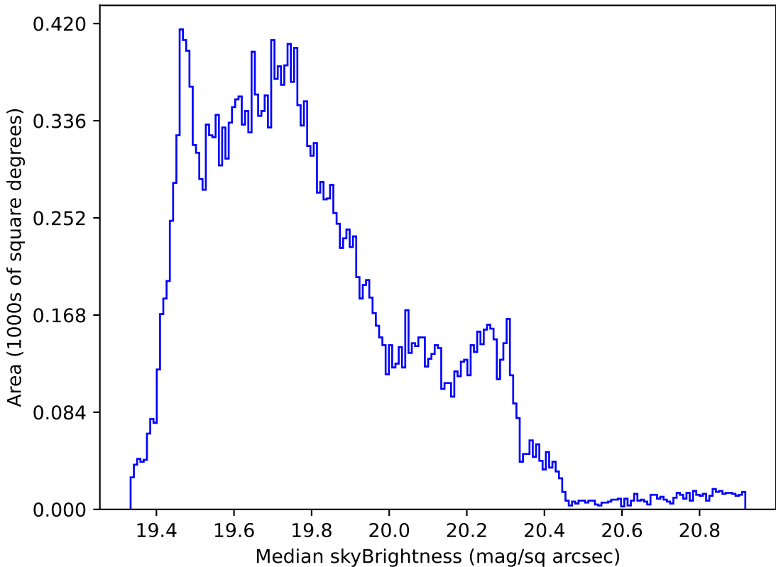
smc_lmc_v3.3_10yrs All sky all bands: Median skyBrightness
