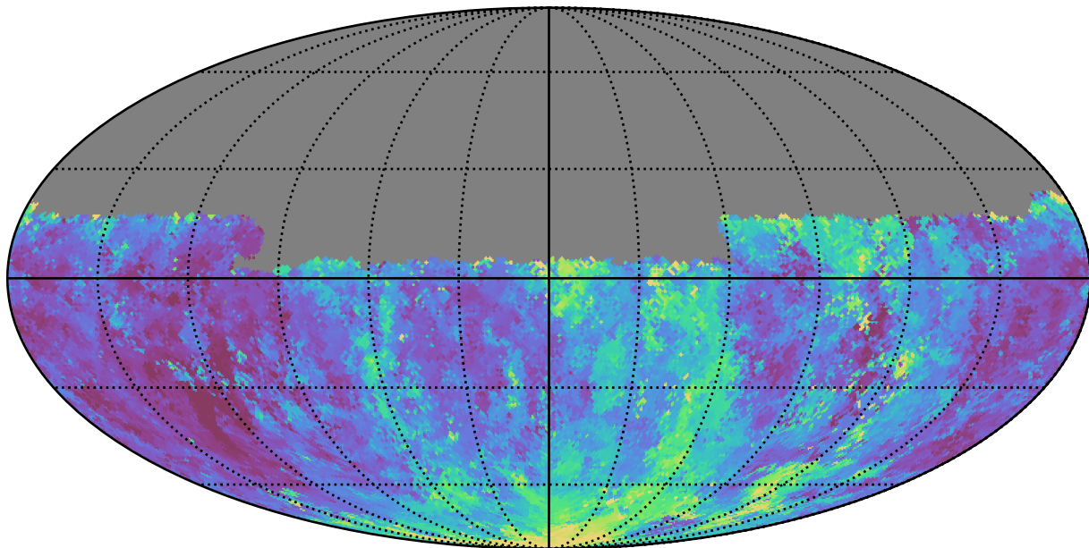
smc_lmc_v3.3_10yrs Yr 1 u band: Median seeingGeom
