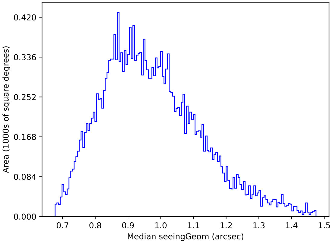
smc_lmc_v3.3_10yrs Yr 1 u band: Median seeingGeom
