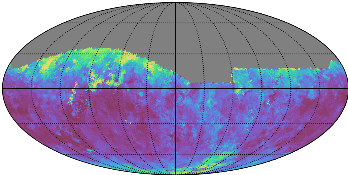
smc_lmc_v3.3_10yrs Yr 1 i band: Median seeingGeom
