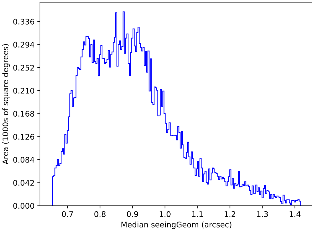
smc_lmc_v3.3_10yrs Yr 1 g band: Median seeingGeom
