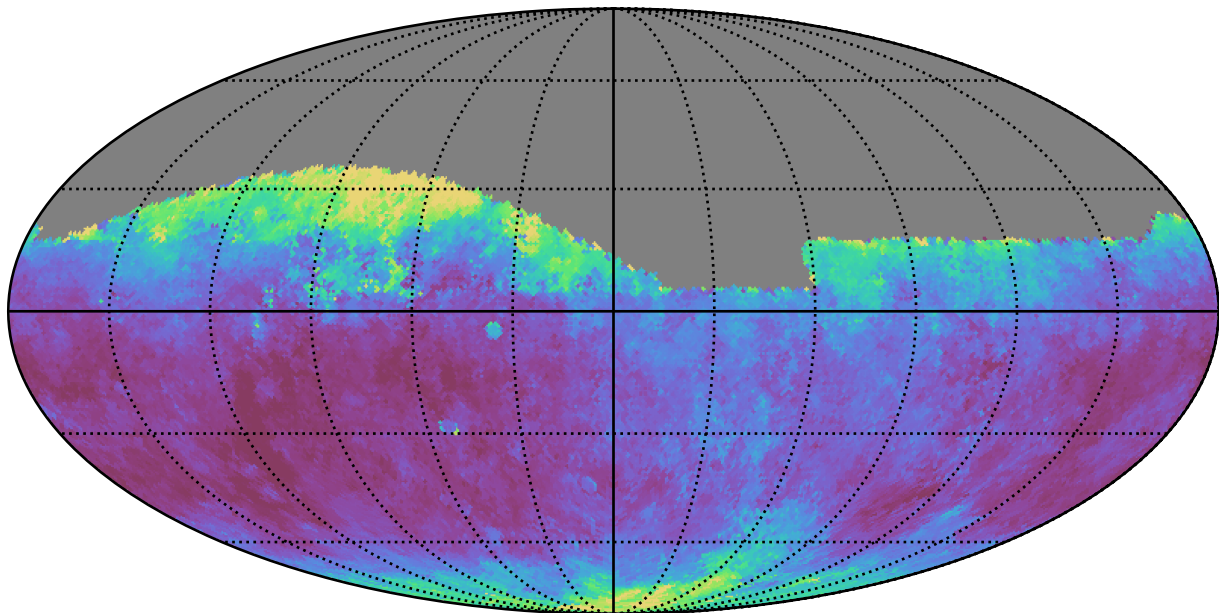
smc_lmc_v3.3_10yrs Yr 1 all bands: Median seeingGeom
