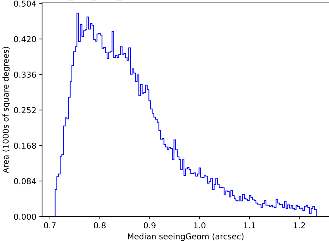
smc_lmc_v3.3_10yrs Yr 1 all bands: Median seeingGeom
