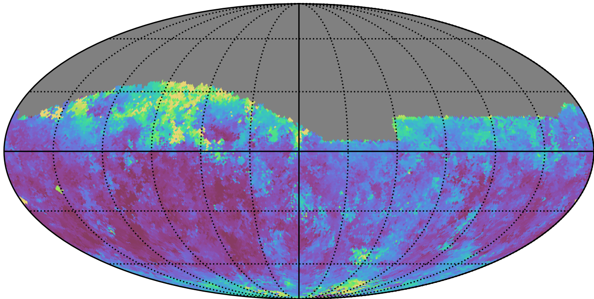
smc_lmc_v3.3_10yrs Yr 1 z band: Median seeingEff
