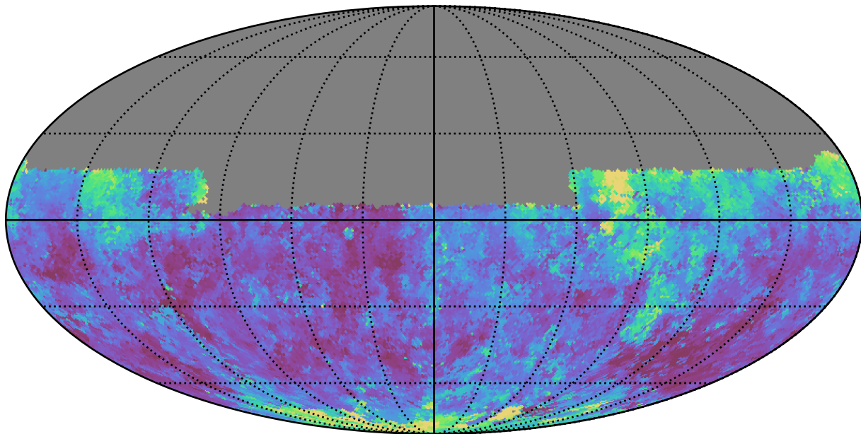
smc_lmc_v3.3_10yrs Yr 1 y band: Median seeingEff
