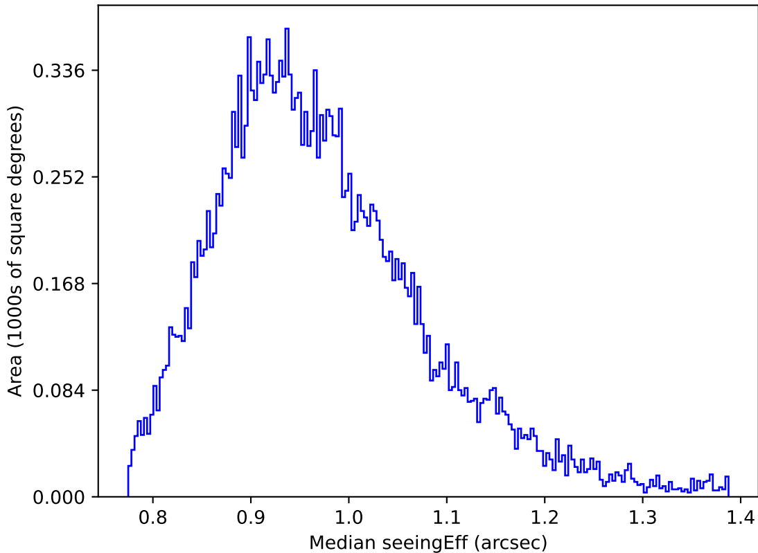
smc_lmc_v3.3_10yrs Yr 1 y band: Median seeingEff
