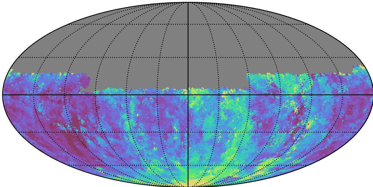
smc_lmc_v3.3_10yrs Yr 1 u band: Median seeingEff
