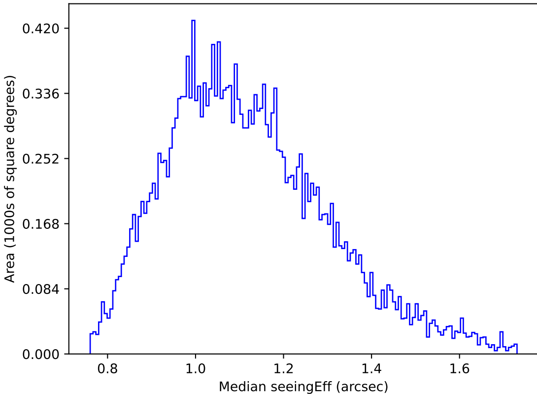
smc_lmc_v3.3_10yrs Yr 1 u band: Median seeingEff
