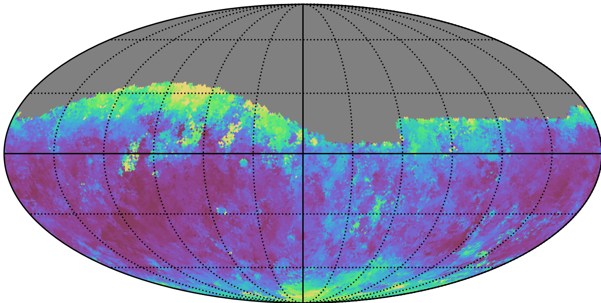
smc_lmc_v3.3_10yrs Yr 1 r band: Median seeingEff
