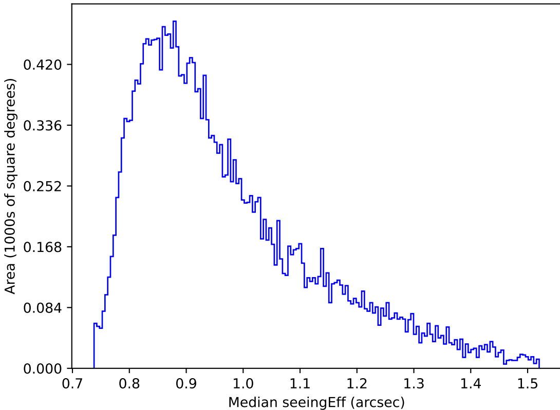
smc_lmc_v3.3_10yrs Yr 1 r band: Median seeingEff
