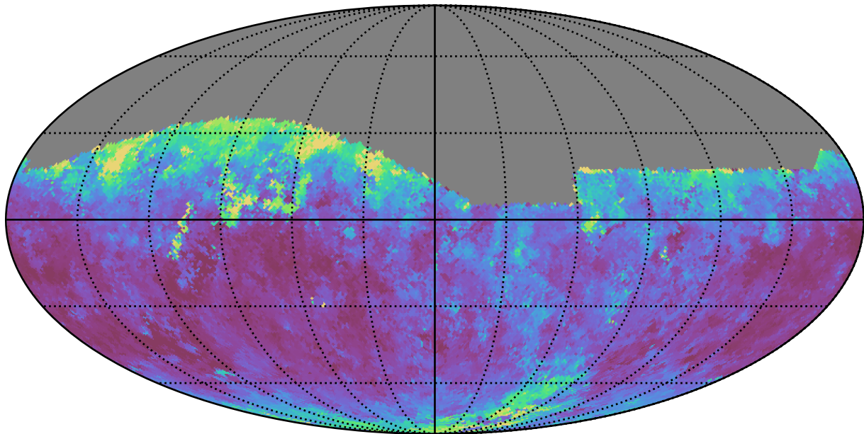
smc_lmc_v3.3_10yrs Yr 1 i band: Median seeingEff
