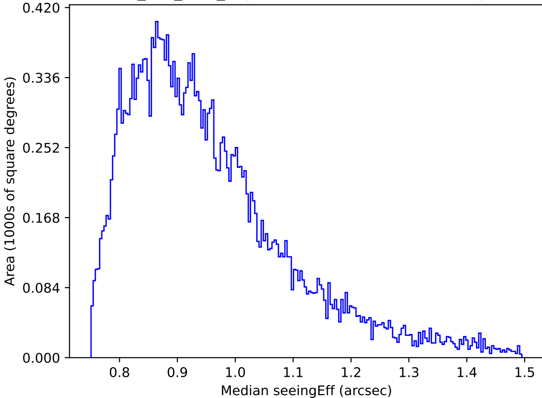
smc_lmc_v3.3_10yrs Yr 1 i band: Median seeingEff
