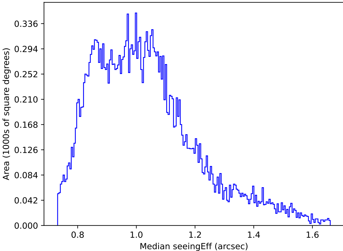
smc_lmc_v3.3_10yrs Yr 1 g band: Median seeingEff
