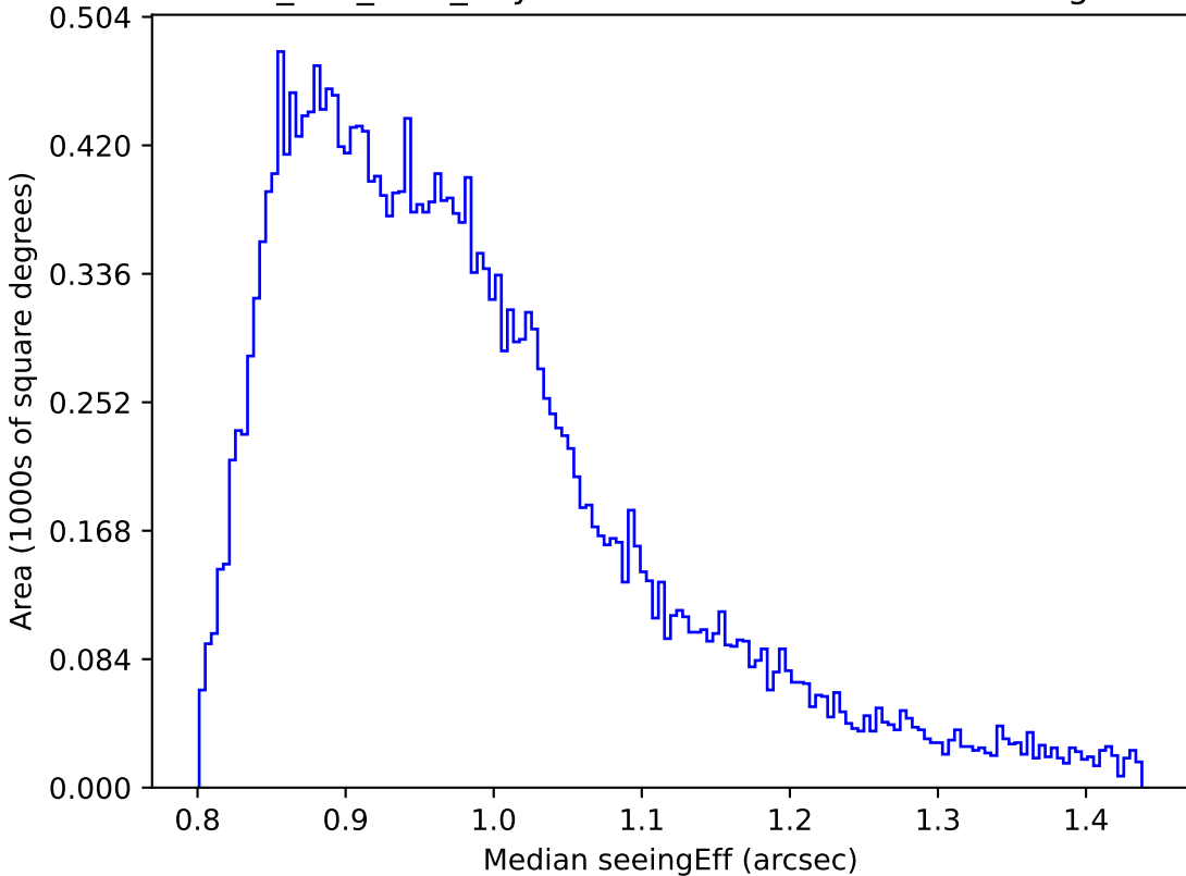
smc_lmc_v3.3_10yrs Yr 1 all bands: Median seeingEff
