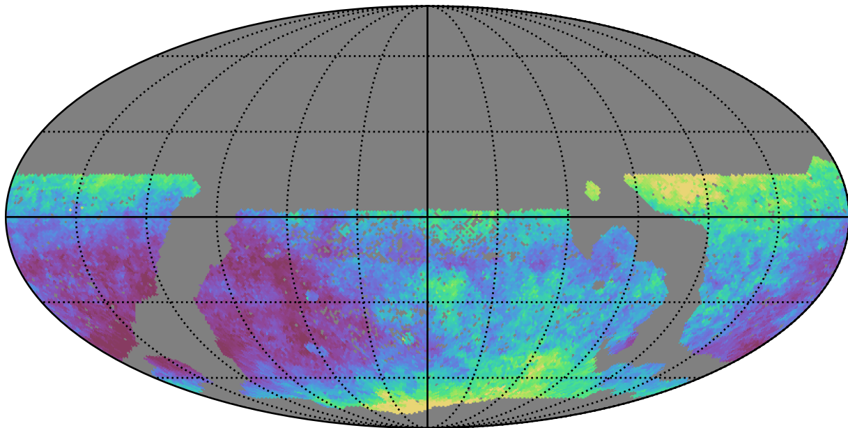
smc_lmc_v3.3_10yrs WFD z band: Median seeingEff
