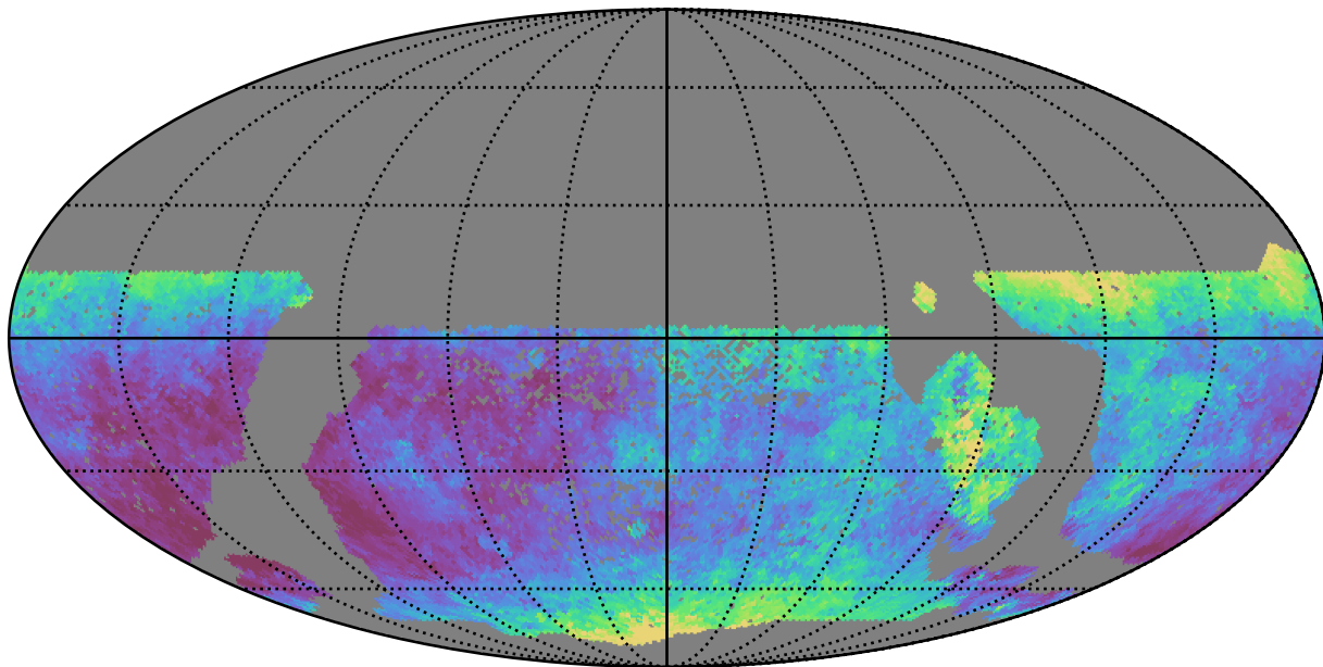
smc_lmc_v3.3_10yrs WFD y band: Median seeingEff
