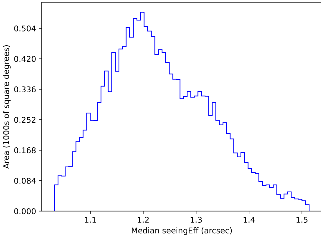
smc_lmc_v3.3_10yrs WFD u band: Median seeingEff
